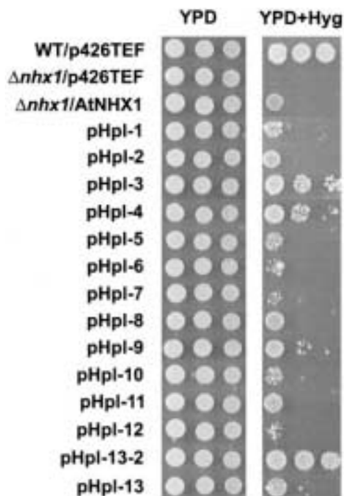
Fig. 2. Complementation test for hygromycin sensitivity of 3xHA-tagged constructs in S. cerevisiae \Delta nhx1 strain. The p426-TEF empty vector was introduced into MM476 (WT/p426TEF) and TY001 ( \Delta nhx1 /p426TEF). p426-X1 ( \Delta nhx1 /AtNHX1) and pHpl constructs (1–13.2) were transformed into TY001 (pHpl-1 to 13.2). Each strain was grown, and serial dilutions were made as described in Materials and Methods . Three microliters of each dilution (starting from 10^6 cells) were spotted onto YPD medium and incubated 2 days at 30^\circ\text{C} , or onto YPD containing 30\ \mu\text{g/ml} hygromycin (YPD+Hyg) and incubated 3 days at 30^\circ\text{C} .
