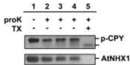
Fig. 3. Vacuolar integrity tests. Intact vacuoles were isolated as described in Materials and Methods . Western blot was performed with anti-CPY antibodies (Upper) or anti-AtNHX1 (Lower). Vacuoles from yeast harboring the pHpl-2 plasmid were incubated with (lanes 2–5) or without (lane 1) 500\ \mu\text{g/ml} proteinase K in the presence (lane 5) or absence (lanes 1–4) of Triton X-100. Untreated control vacuoles (lane 1) and vacuoles containing proteinase K and Triton X-100 (lane 5) were incubated for 90 min on ice. Vacuoles containing proteinase K only (lanes 2–4) were incubated for 30 min (lane 2), 60 min (lane 3), and 90 min (lane 4) on ice, respectively.
