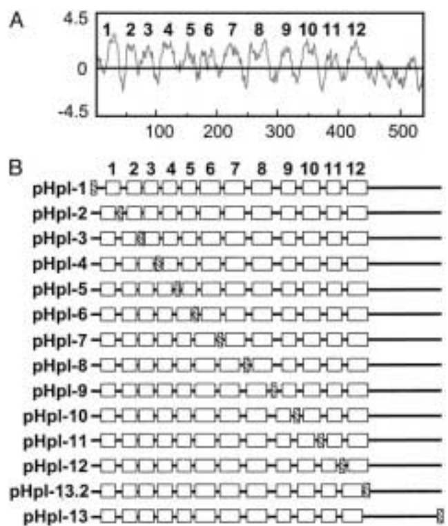
Fig. 1. HA-tagged constructs of AtNHX1. (A) Hydropathy plot of AtNHX1. (B) Schematic diagram indicating the 3xHA-tagged AtNHX1 constructs used in this study. Numerals above the boxes indicate the number of putative transmembrane domains. Blank boxes indicate putative transmembrane domains and shadowed box indicates 3xHA-tag.
